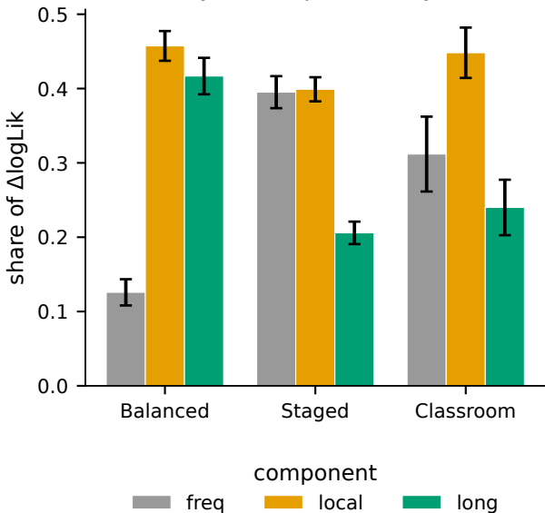
Predictability decomposition by curriculum
